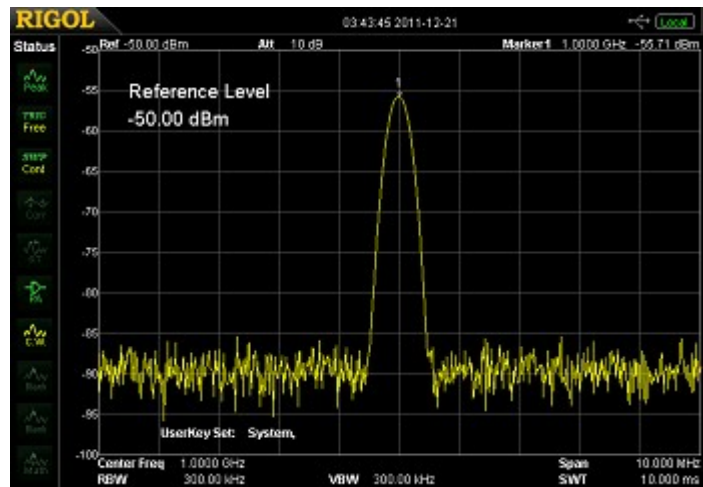
Figure 2: Preamplifier on
