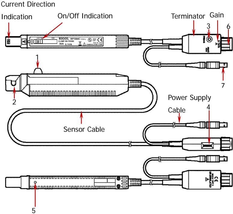
Figure 2 RP1004C Parts
